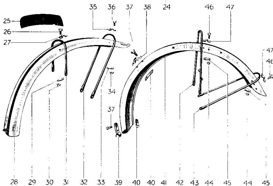
FRONT AND REAR MUDGUARDS
