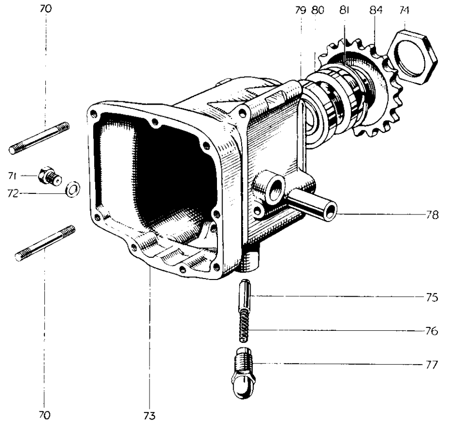
TRIUMPH FOUR SPEED GEARBOX
