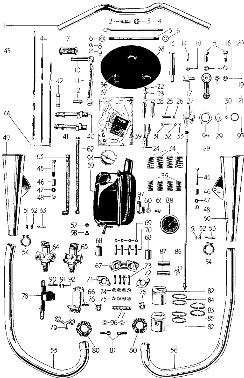
T100 RACING KIT
