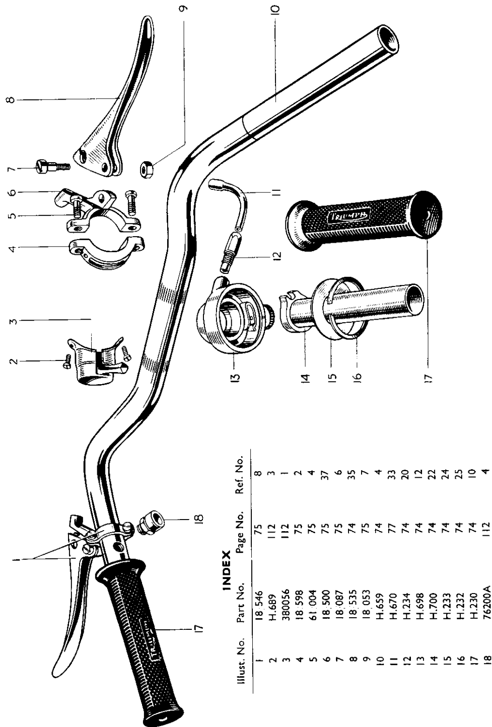
HANDLEBAR AND CONTROLS—5T, 6T AND T100
