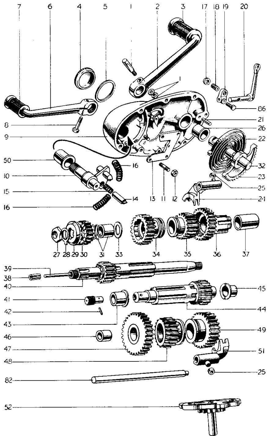
TRIUMPH FOUR SPEED GEARBOX
