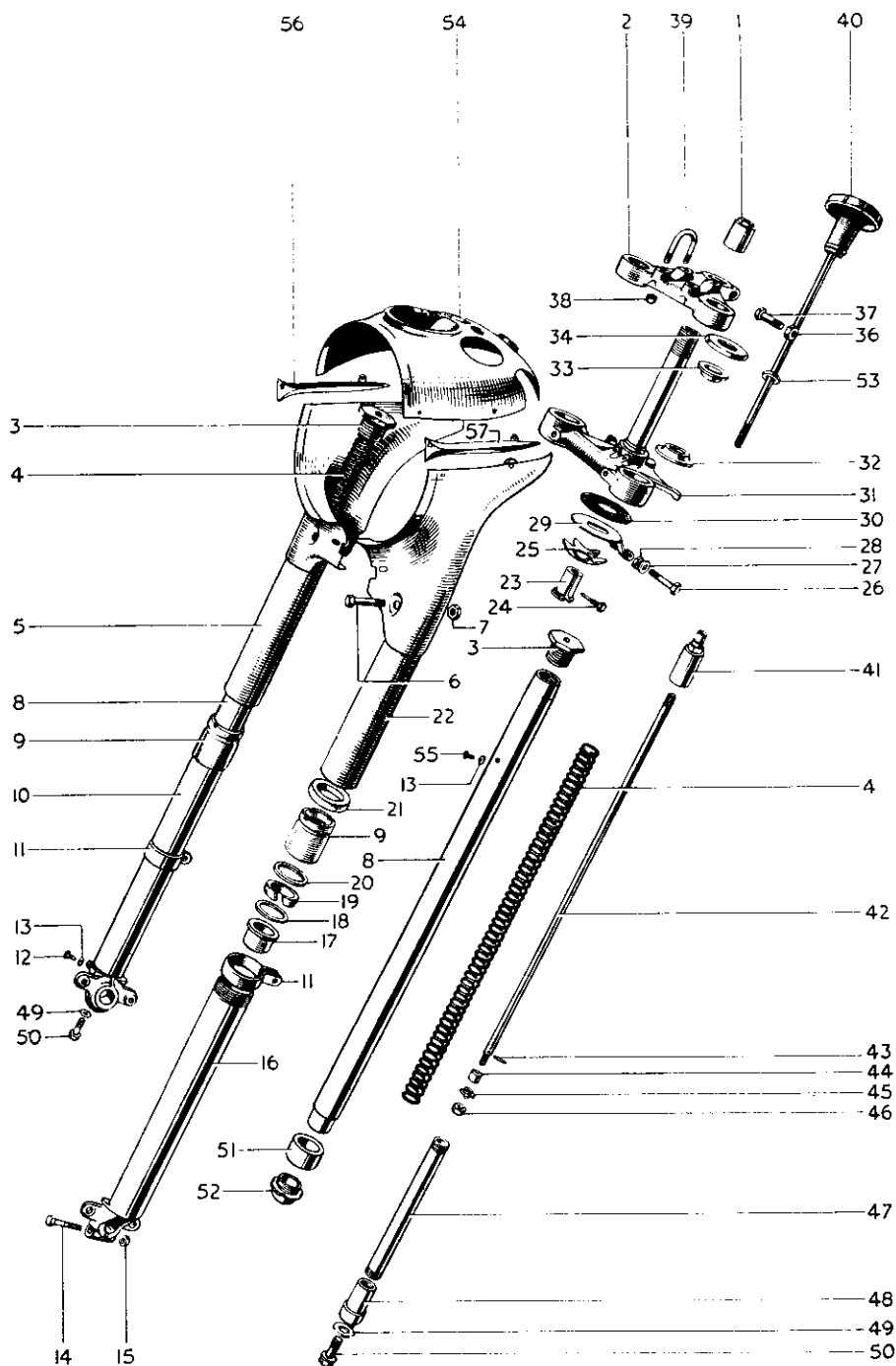
5T, 6T AND T100 TELESCOPIC FORK
