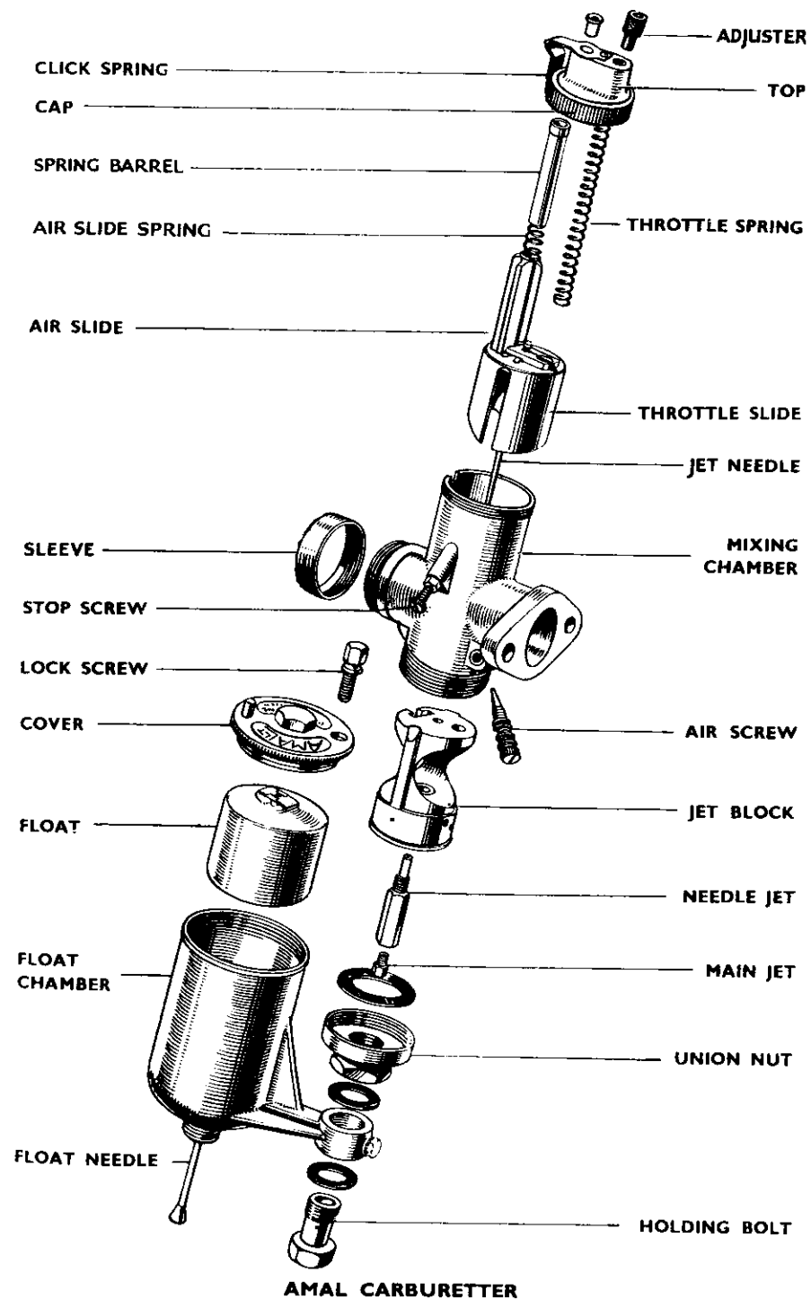
AMAL CARBURETTER
