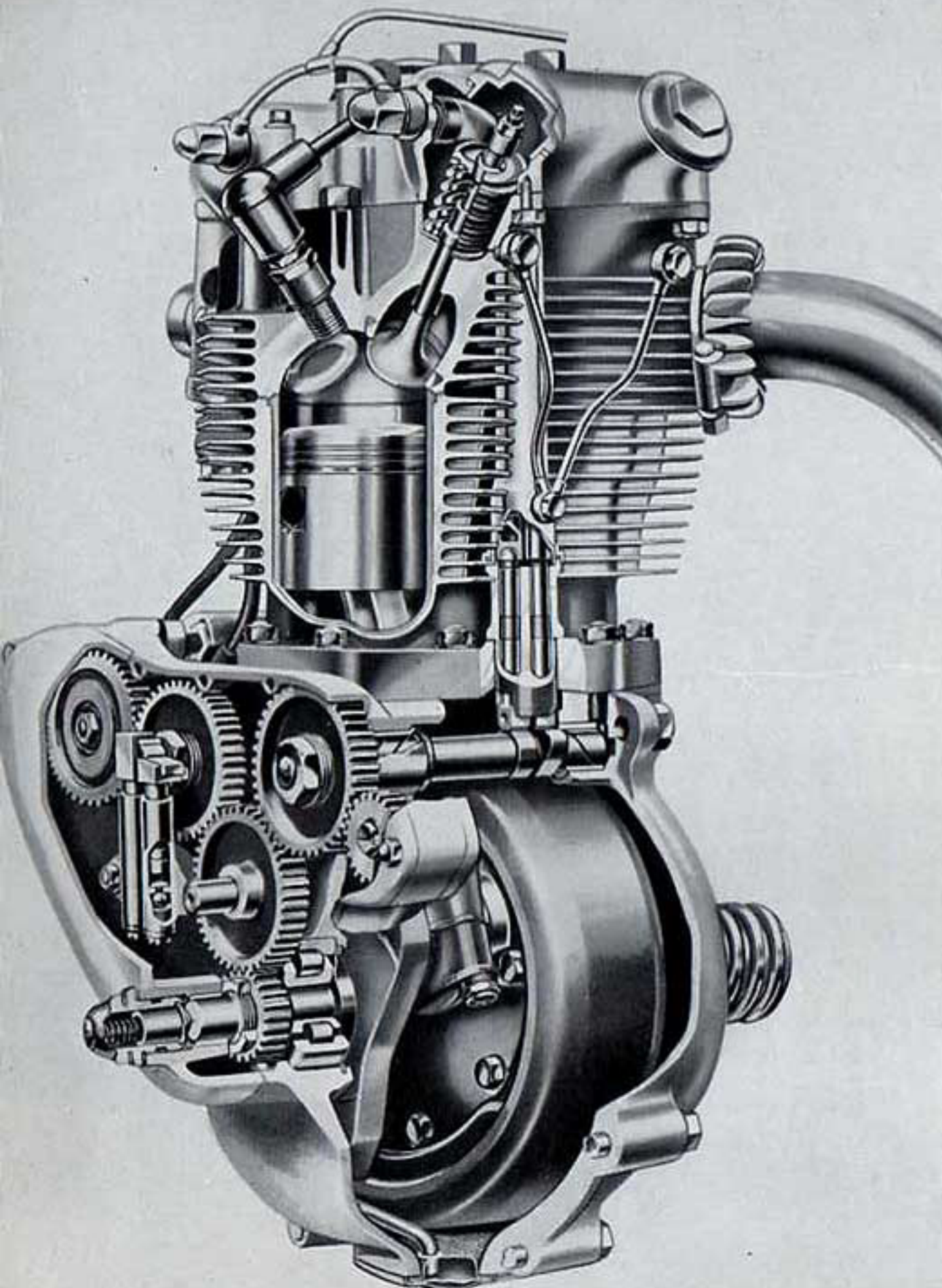
Sectional View Tiger 100 Engine.
